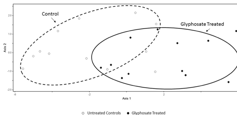
Fig. 1. Principal component analysis (PCA) plot of microbial phospholipid fatty acid (PLFA) profiles derived from rhizosphere soil of control (open symbols) and glyphosate-treated (closed symbols) plants. Variance of the data explained Axis 1: 70.5%, Axis 2: 8.1%. Circles on plot represent treatment groupings for control (dashed circle) and glyphosate-treated (solid circle) samples.
