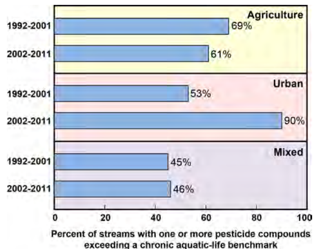
Figure 4. Proportion of streams with one or more pesticides that exceeded a chronic aquatic-life benchmark was very similar between 1992 and 2001 and 2002–2011 for agricultural and mixed-land-use streams, but much greater during 2002–2011 for urban streams.
